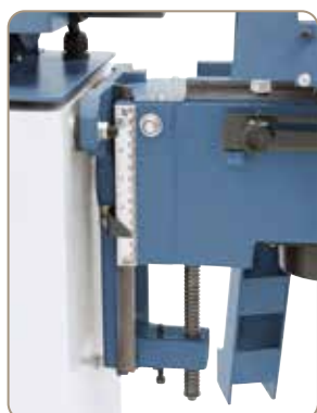
Set height of work table can be read out on scale.
