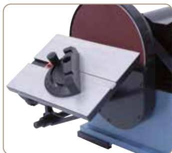
Aluminium support table can be tilted steplessly from 0° - 45°.
