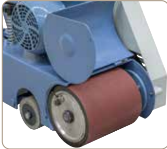
Rubber coated sanding roller features quick clamping system for easy change of sanding belt.
